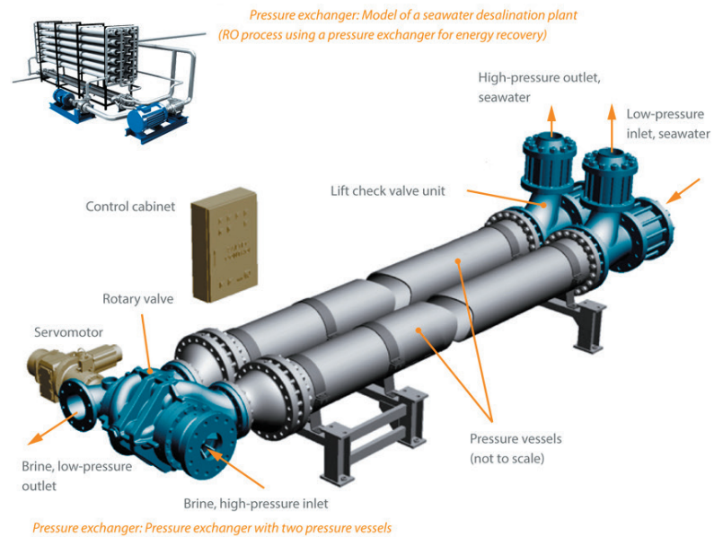
Pressure exchanger: Pressure exchanger with two pressure vessels
